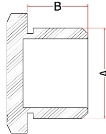
Plug Sets (Plug+'O' Ring +Lock nut)
