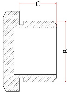
Plug Sets (Plug+'O' Ring +Lock nut)
